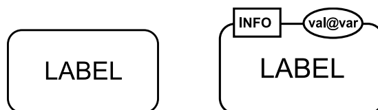
Figure 2.10: The Process Description glyph for macromolecule, shown plain and unadorned on the left, and with with an additional state variable and a unit of information on the right.
