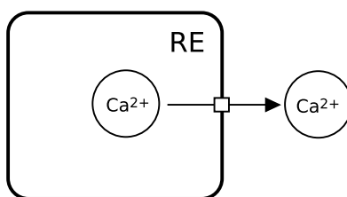
Figure 2.31: A translocation.
