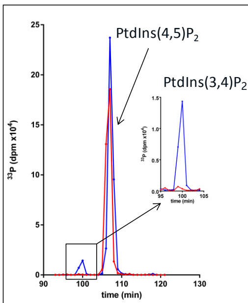
HPLC on anion exchange column
