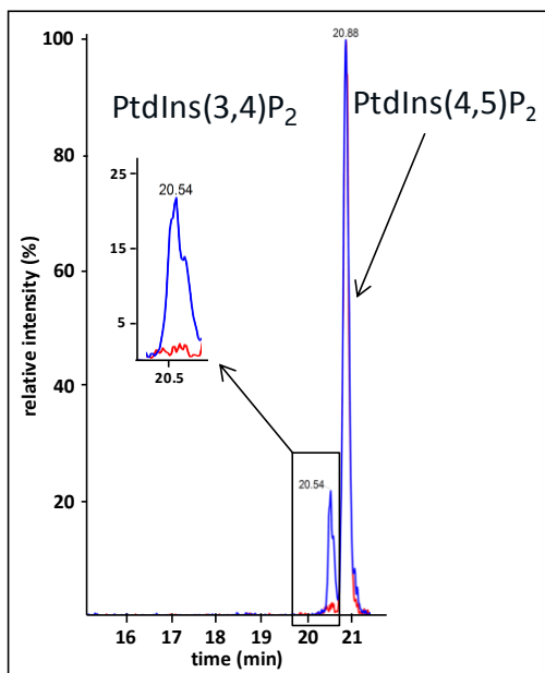
HPLC-MS on C18-column
